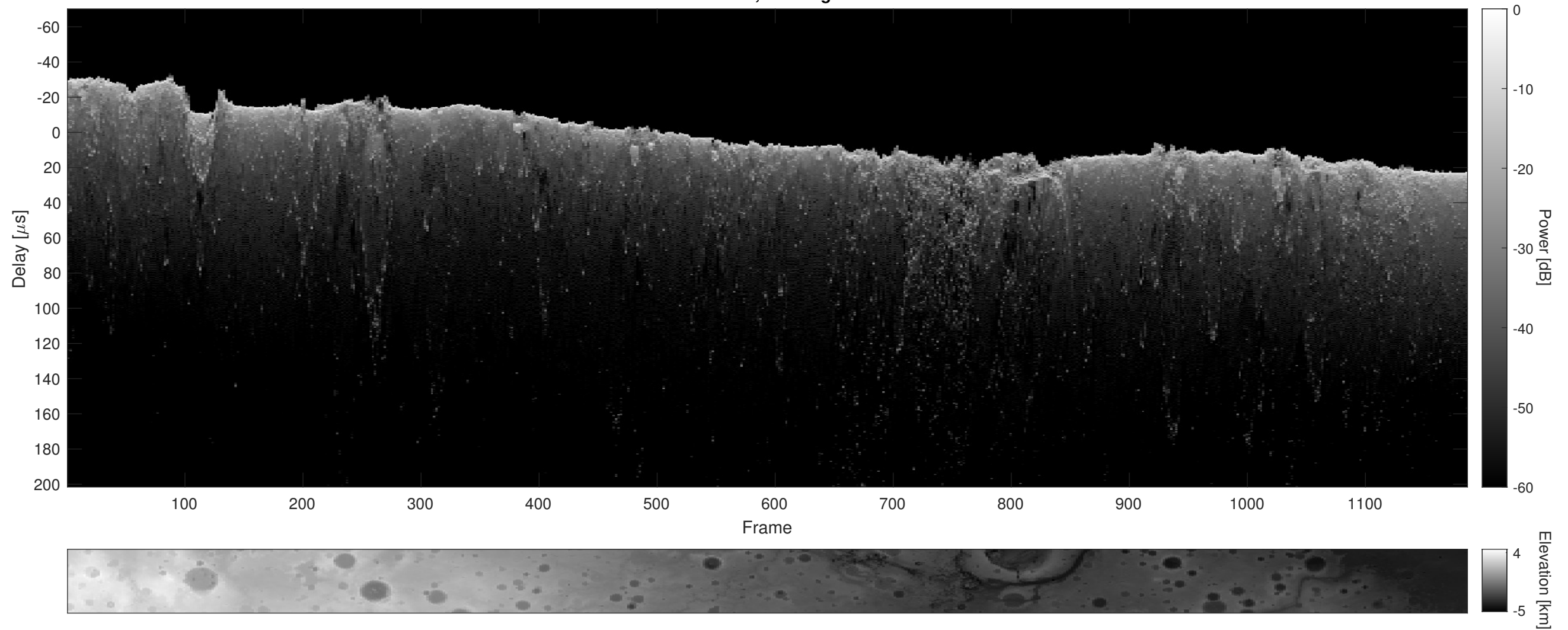
Orbit 8307, Cluttergram
