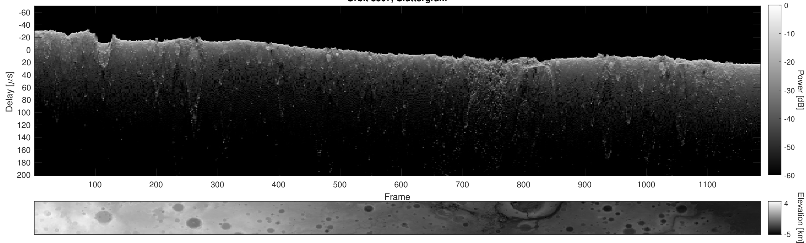
Orbit 8307, Cluttergram
