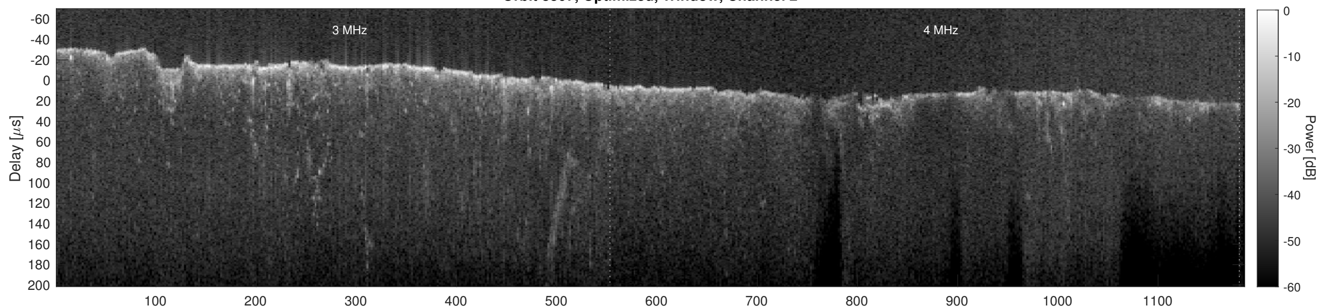
Orbit 8307, Cluttergram
