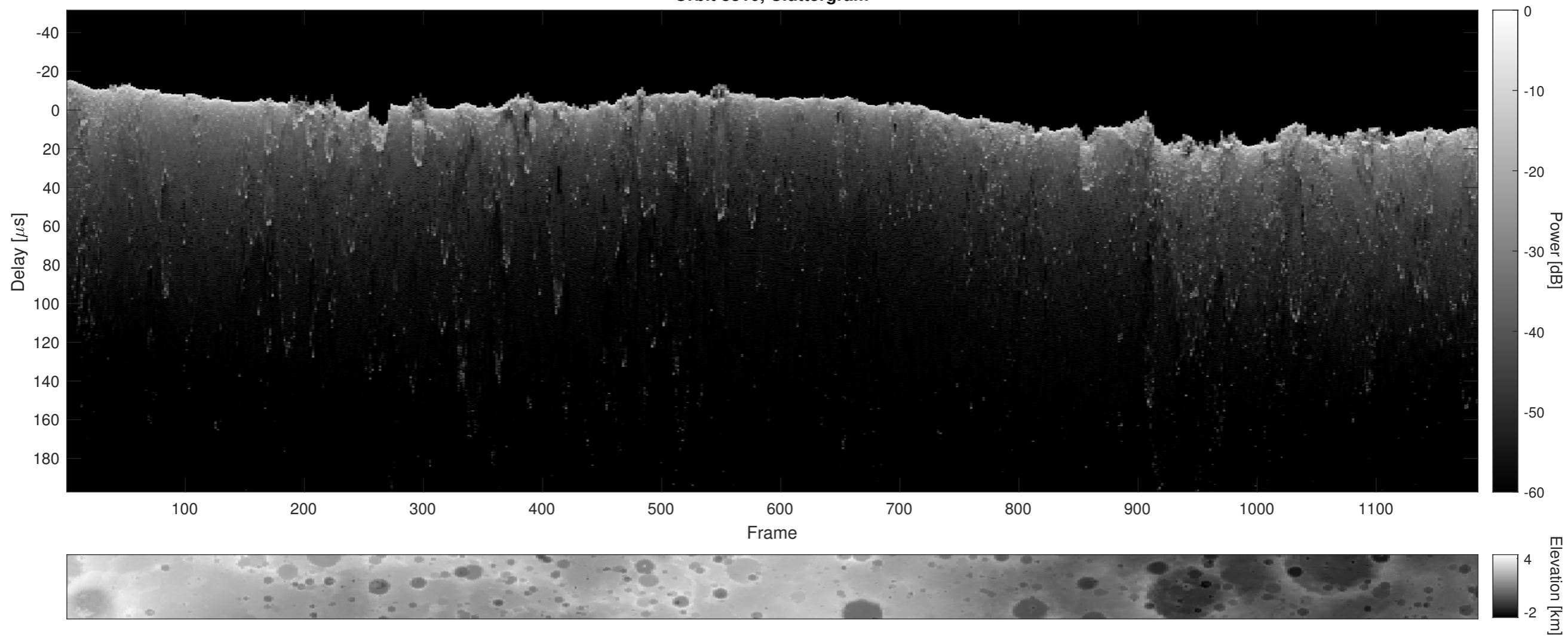
Orbit 8310, Cluttergram
