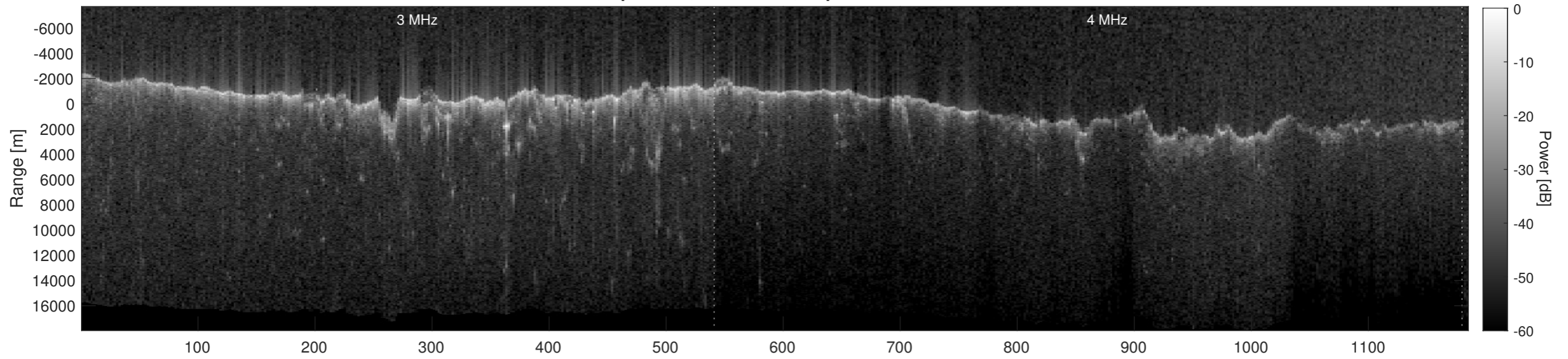
Orbit 8310, Depth-Corrected Cluttergram
