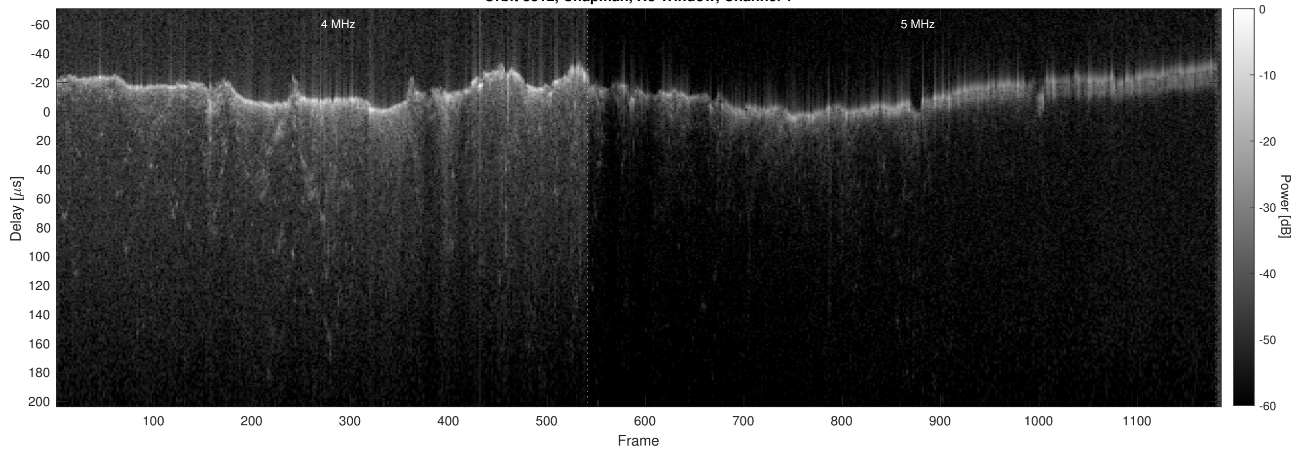
Orbit 8312, Chapman, No Window, Channel 2
