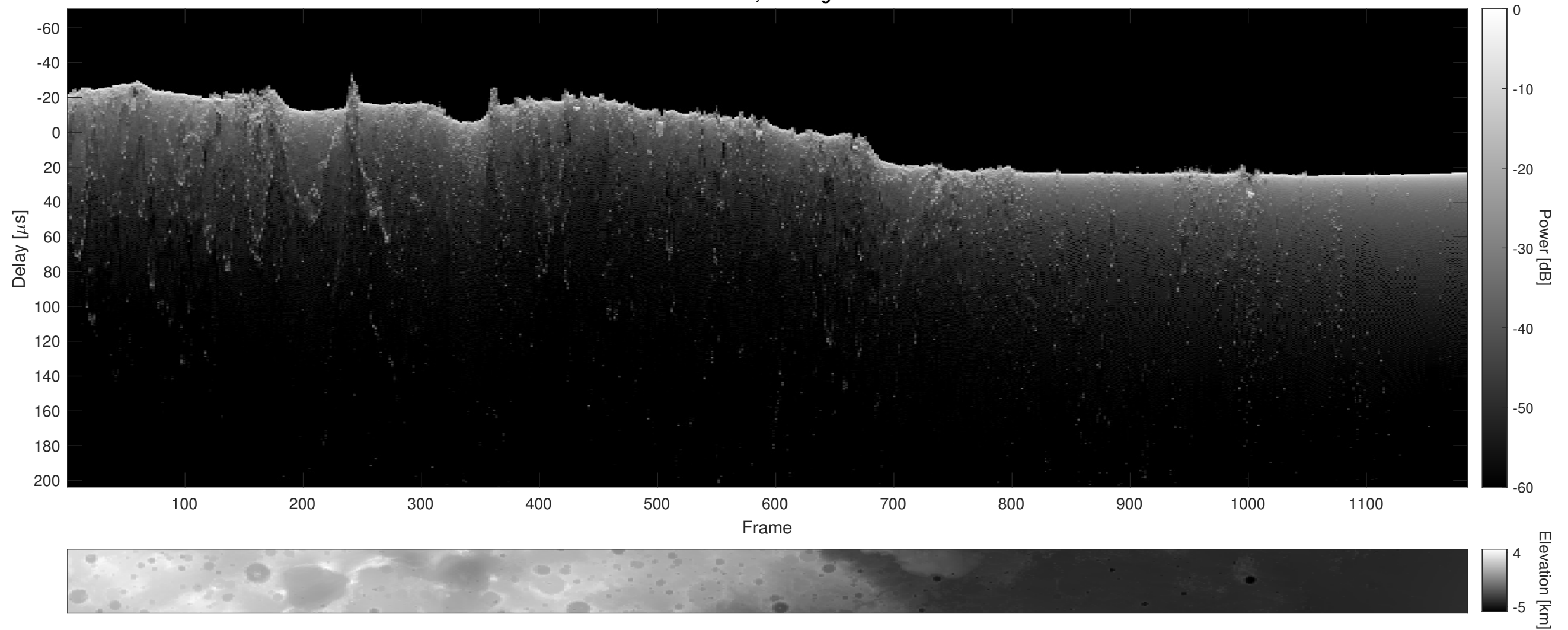
Orbit 8312, Cluttergram
