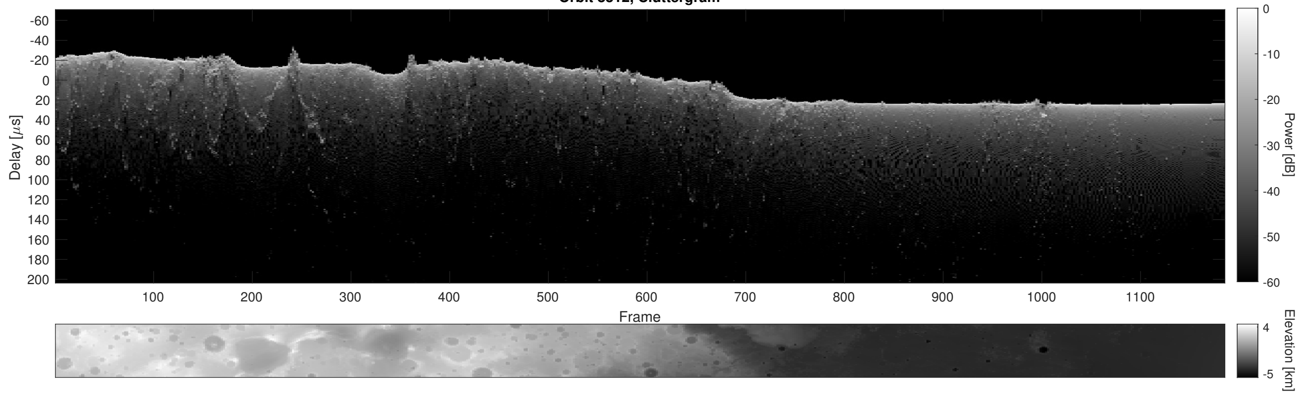
Orbit 8312, Cluttergram
