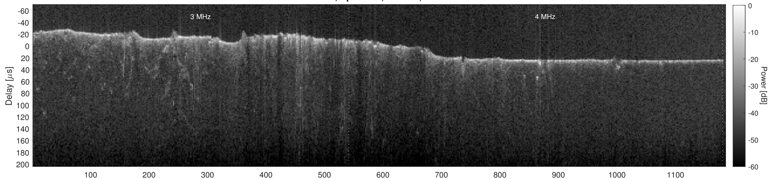
Orbit 8312, Cluttergram
