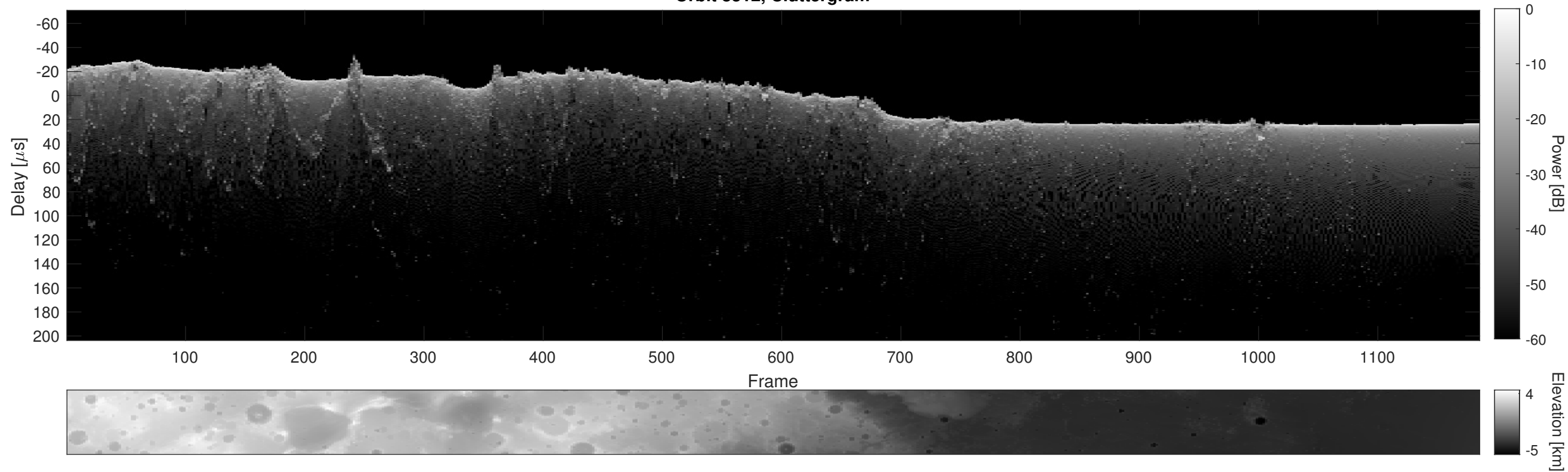
Orbit 8312, Cluttergram
