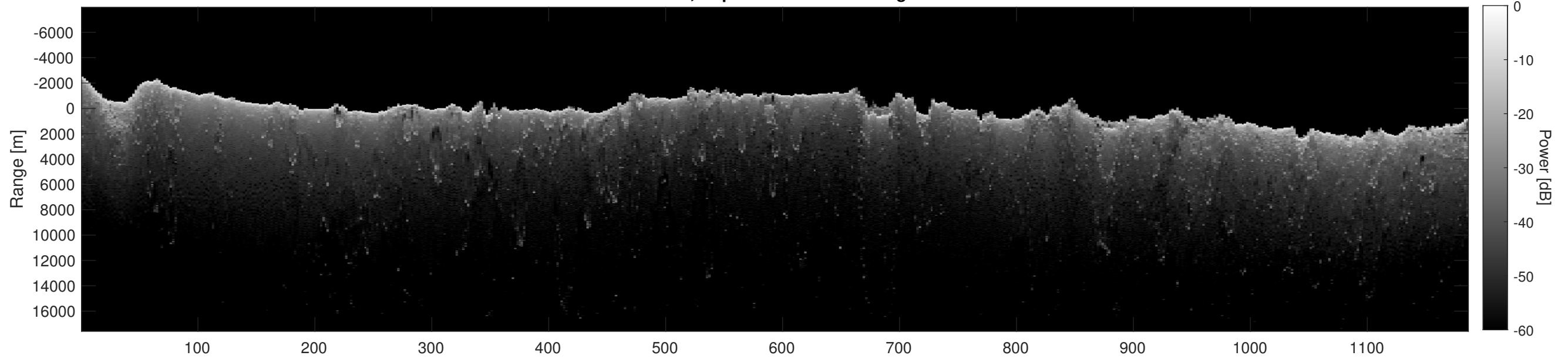
Orbit 8317, Depth-Corrected Cluttergram
