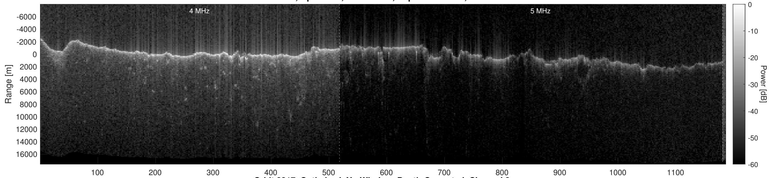
Orbit 8317, Optimized, No Window, Depth-Corrected, Channel 2
