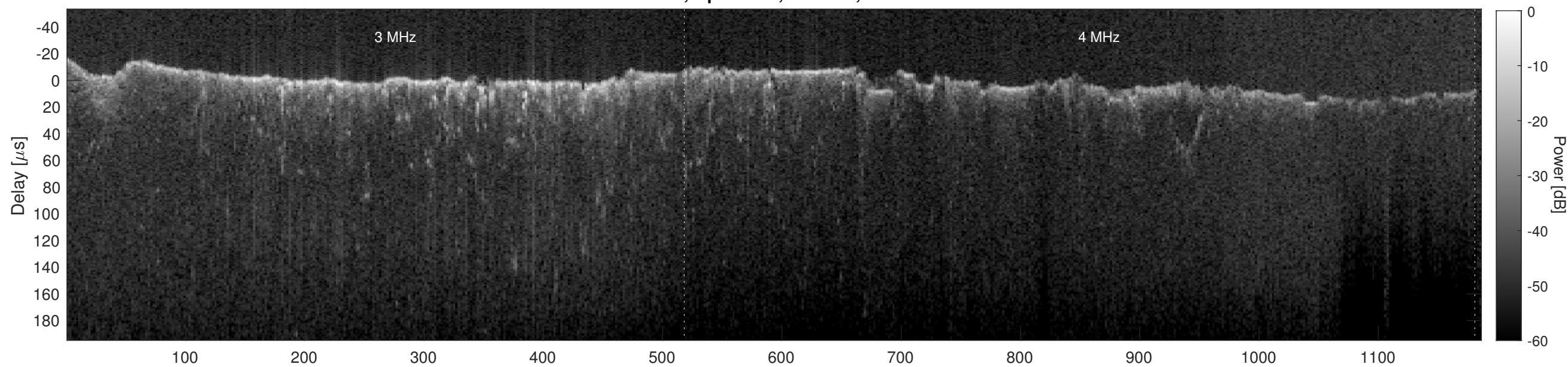
Orbit 8317, Cluttergram
