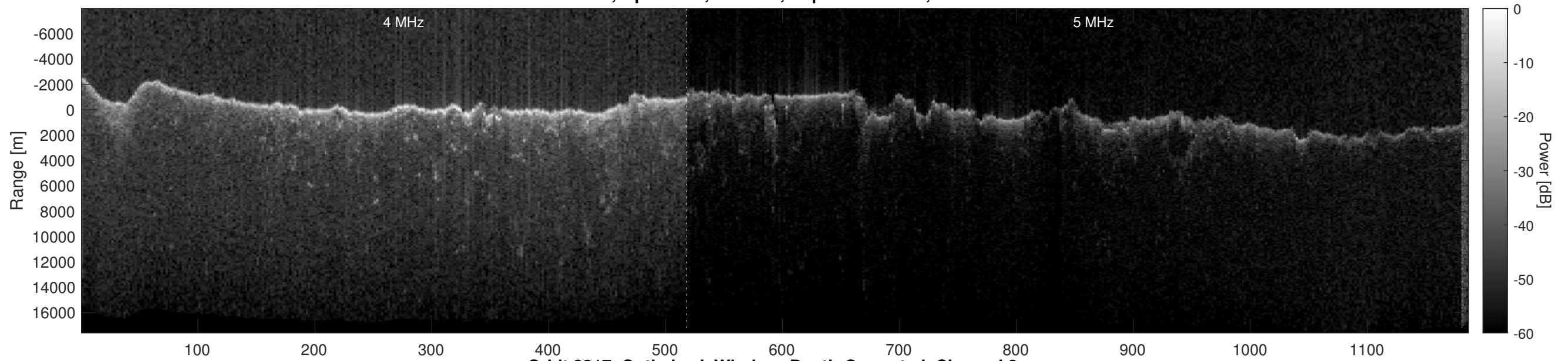
Orbit 8317, Optimized, Window, Depth-Corrected, Channel 2
