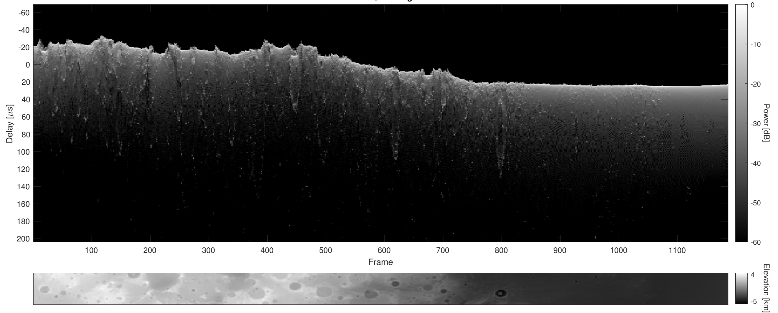
Orbit 8319, Cluttergram
