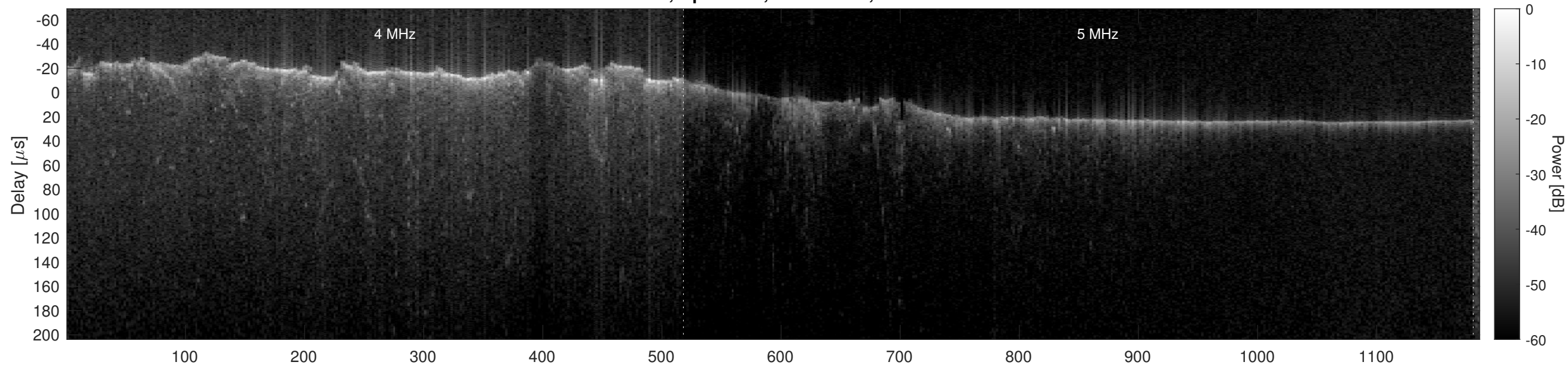
Orbit 8319, Optimized, No Window, Channel 2
