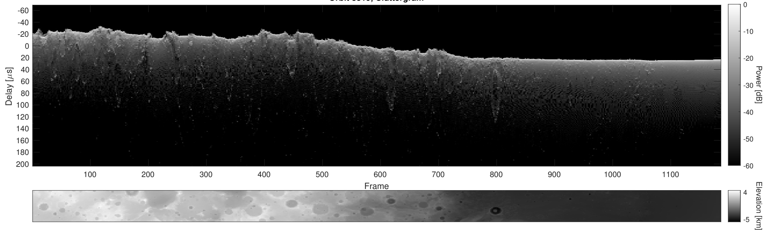
Orbit 8319, Cluttergram
