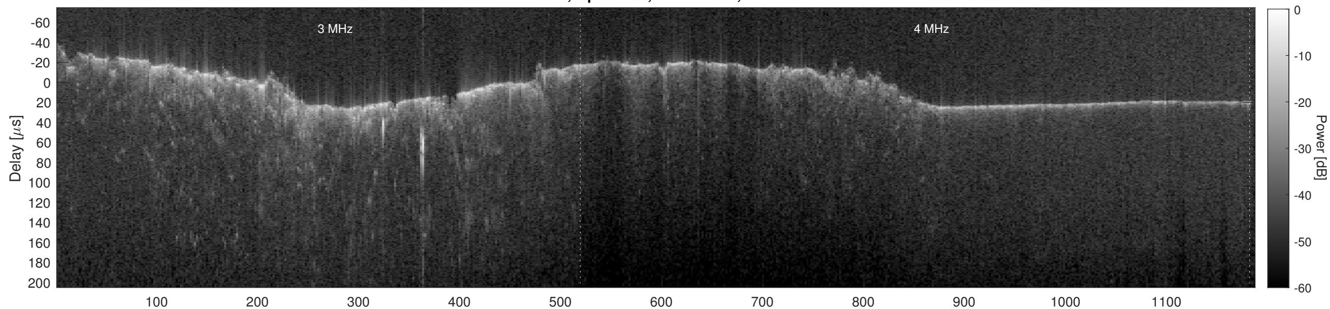
Orbit 8320, Cluttergram
