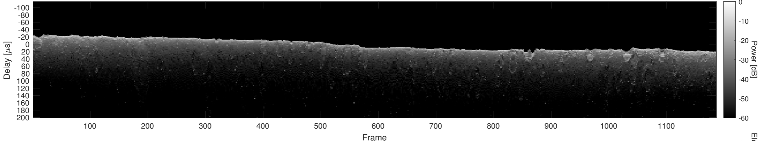
Orbit 8321, Cluttergram
