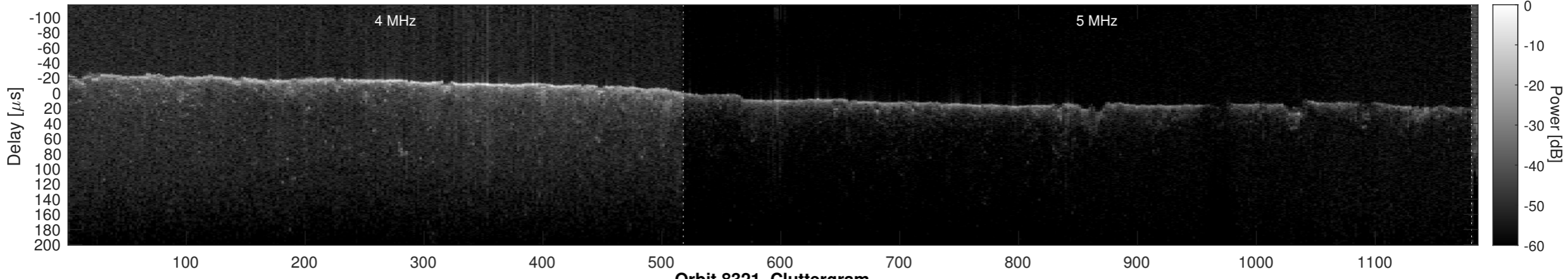
Orbit 8321, Cluttergram
