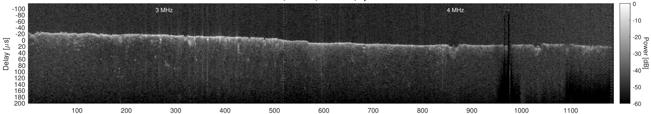
Orbit 8321, Cluttergram
