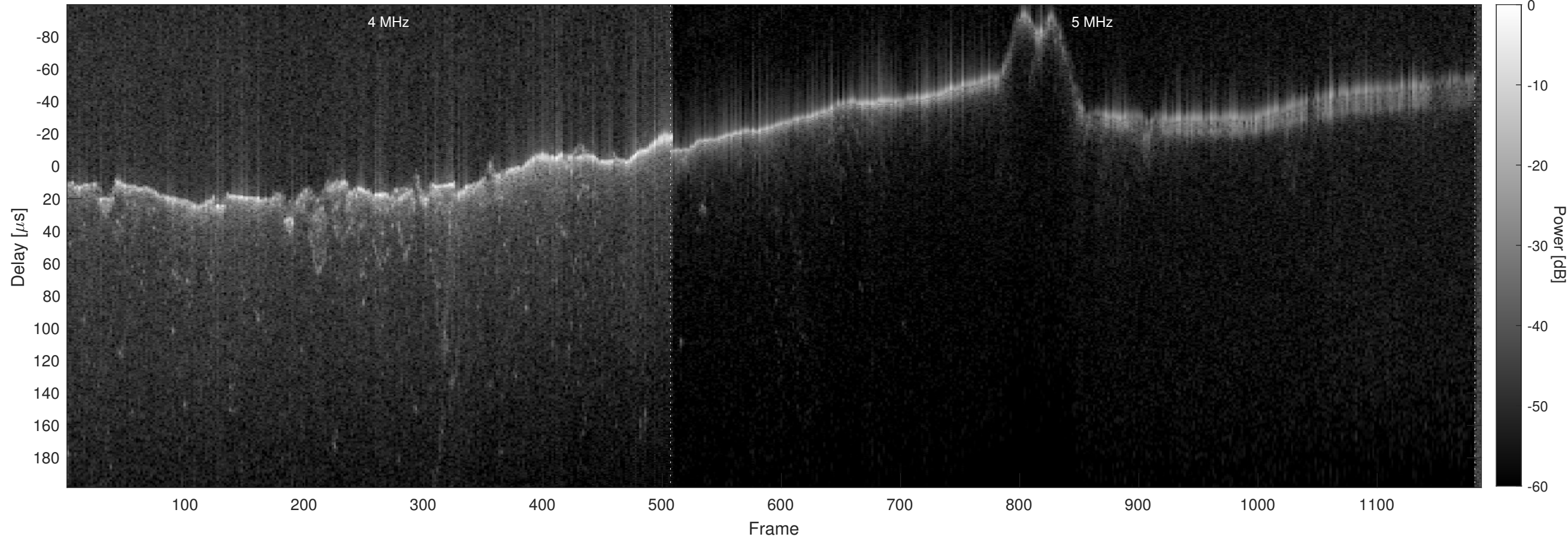
Orbit 8322, Chapman, No Window, Channel 2
