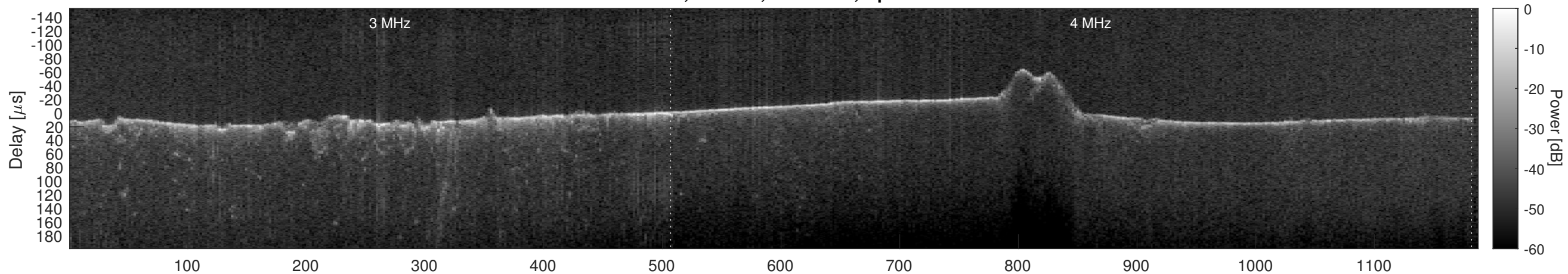
Orbit 8322, Cluttergram
