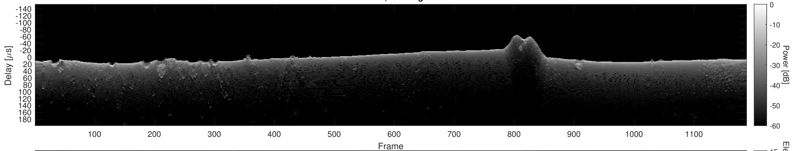
Orbit 8322, Cluttergram
