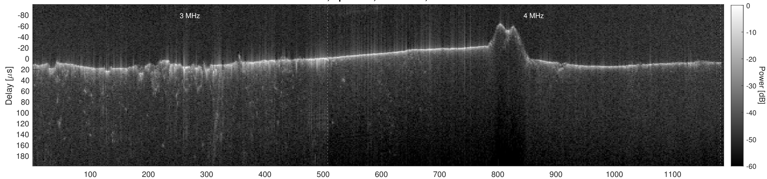
Orbit 8322, Cluttergram
