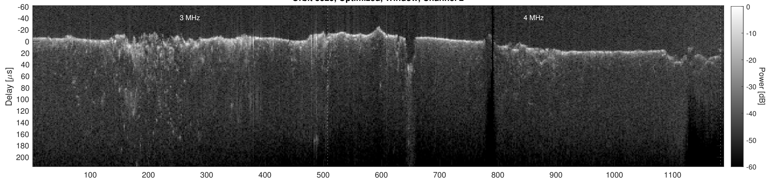
Orbit 8325, Cluttergram
