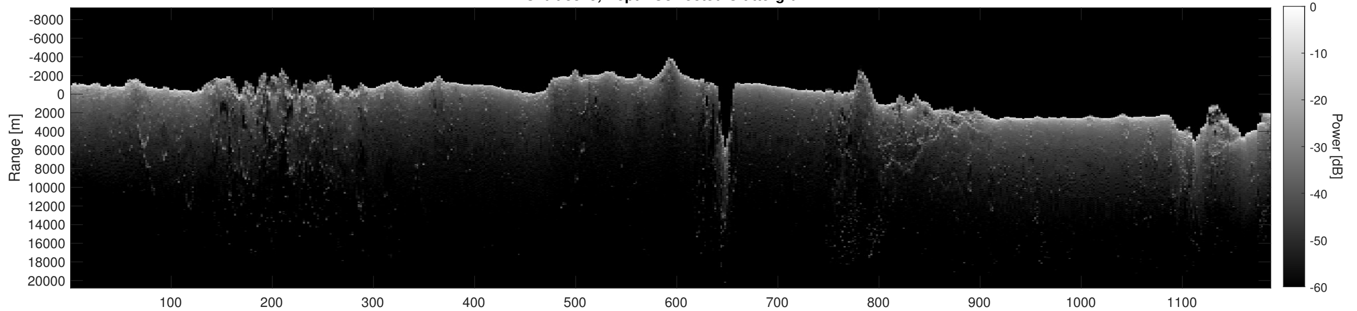
Orbit 8325, Depth-Corrected Cluttergram
