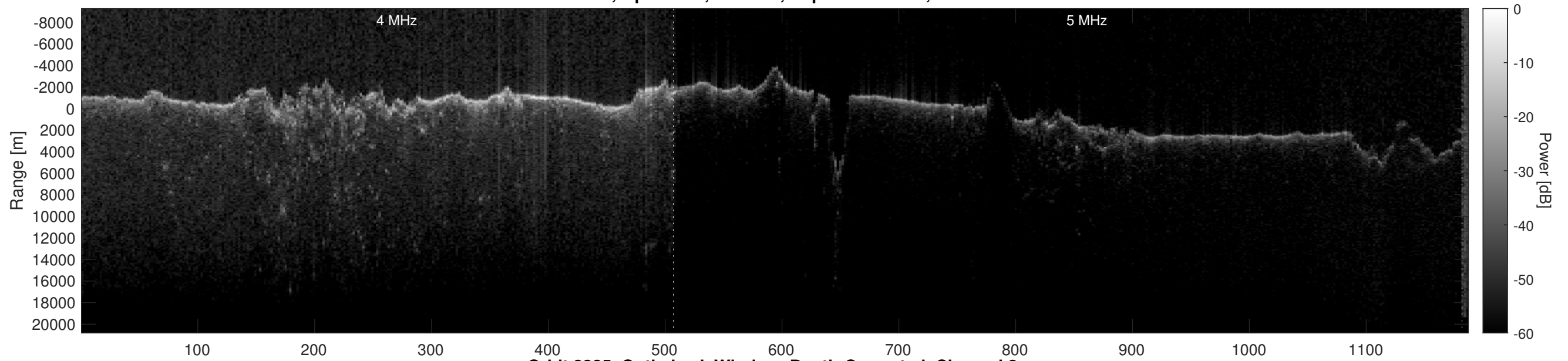
Orbit 8325, Optimized, Window, Depth-Corrected, Channel 2
