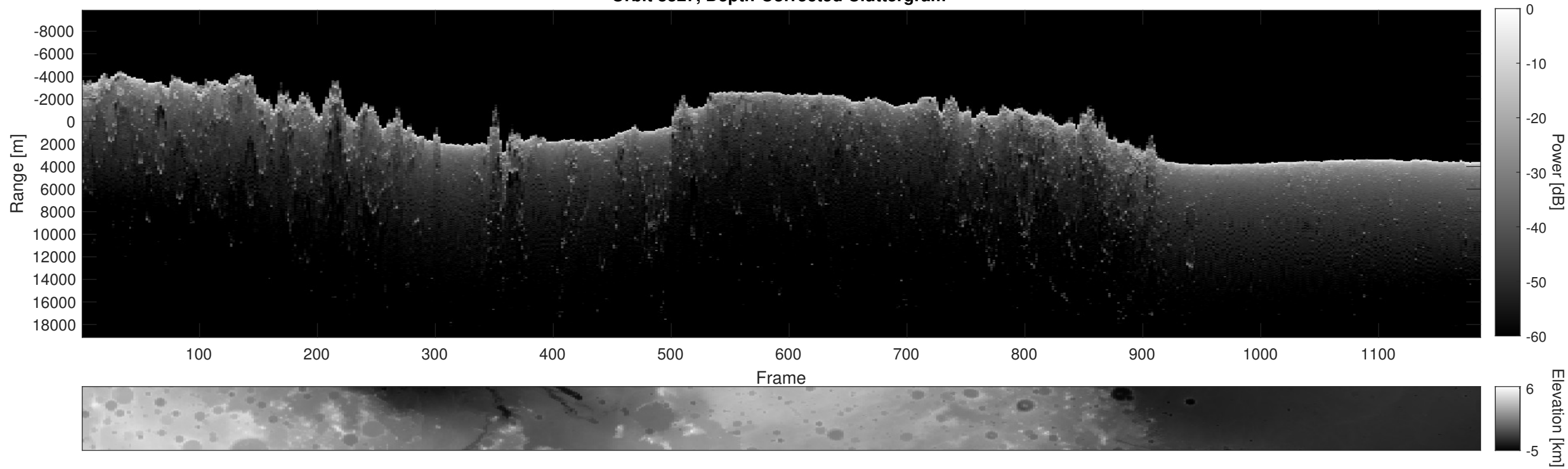
Orbit 8327, Depth-Corrected Cluttergram
