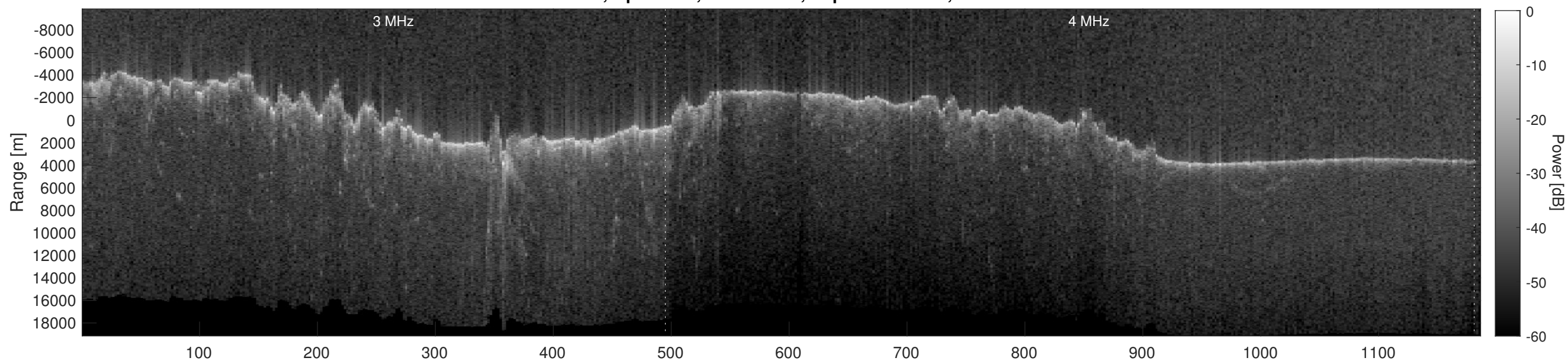
Orbit 8327, Depth-Corrected Cluttergram
