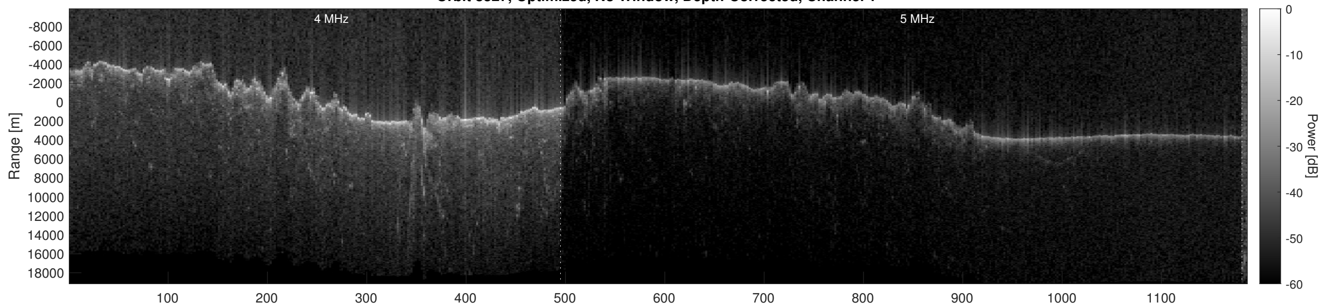
Orbit 8327, Optimized, No Window, Depth-Corrected, Channel 2
