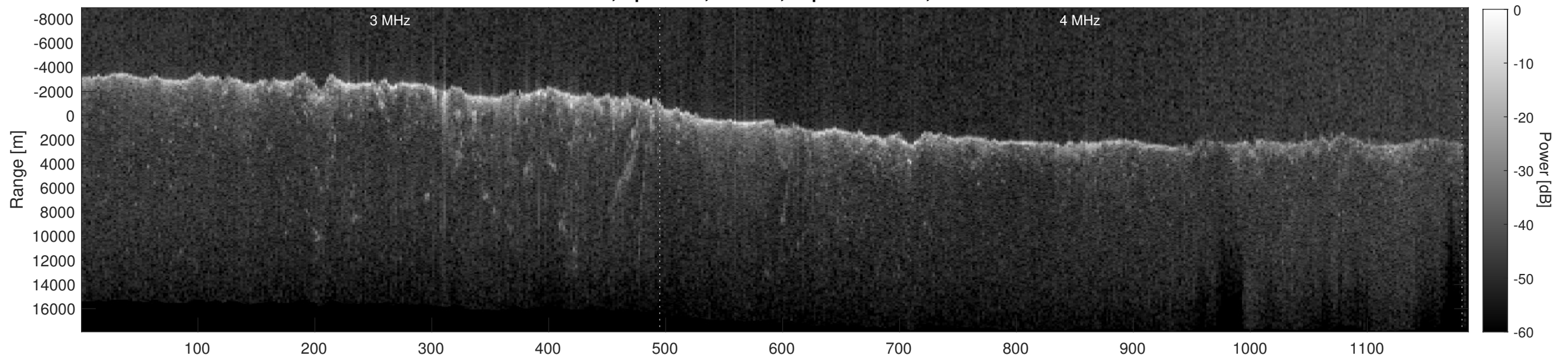
Orbit 8328, Depth-Corrected Cluttergram
