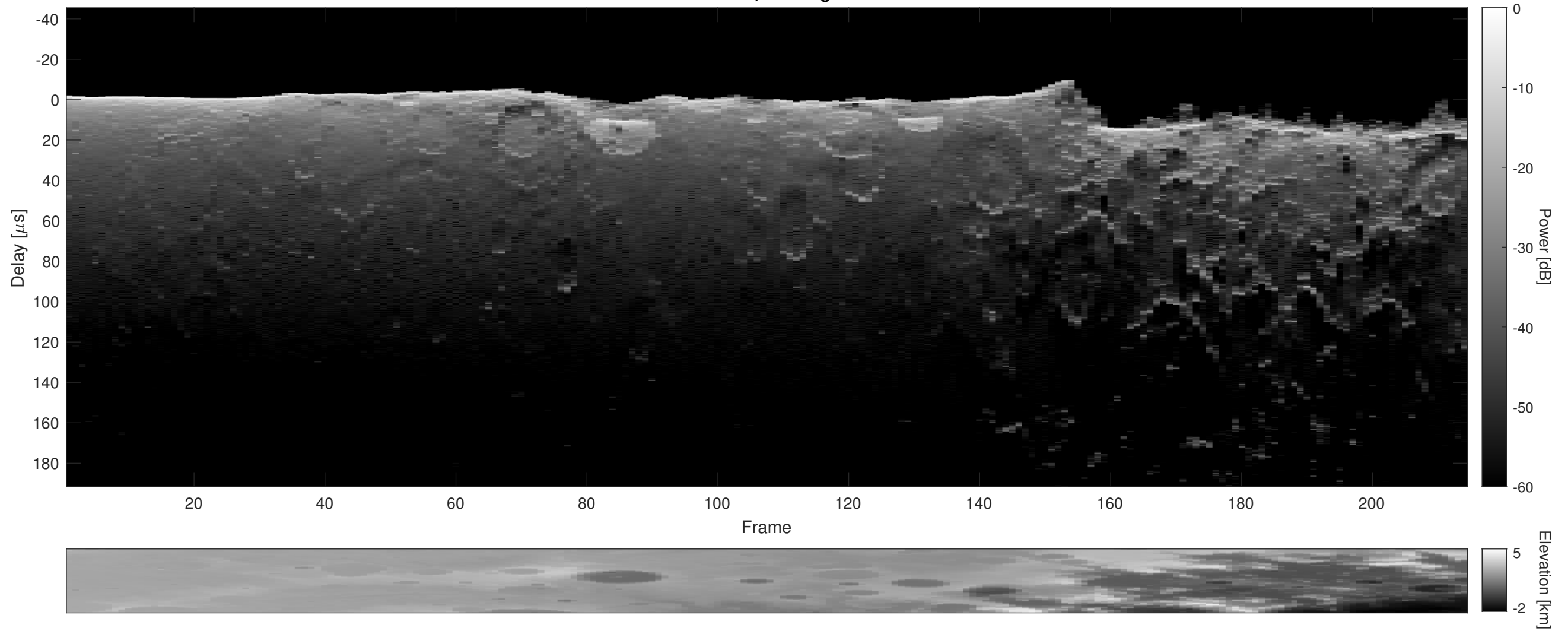
Orbit 8332, Cluttergram
