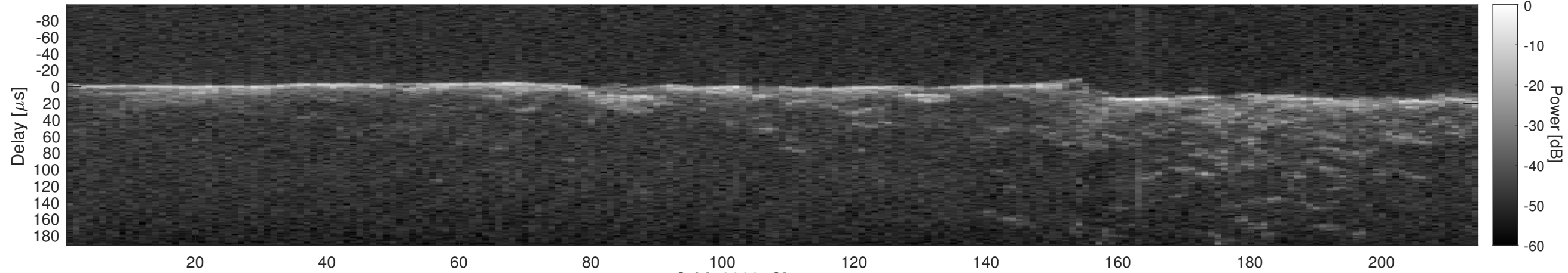
Orbit 8332, Cluttergram
