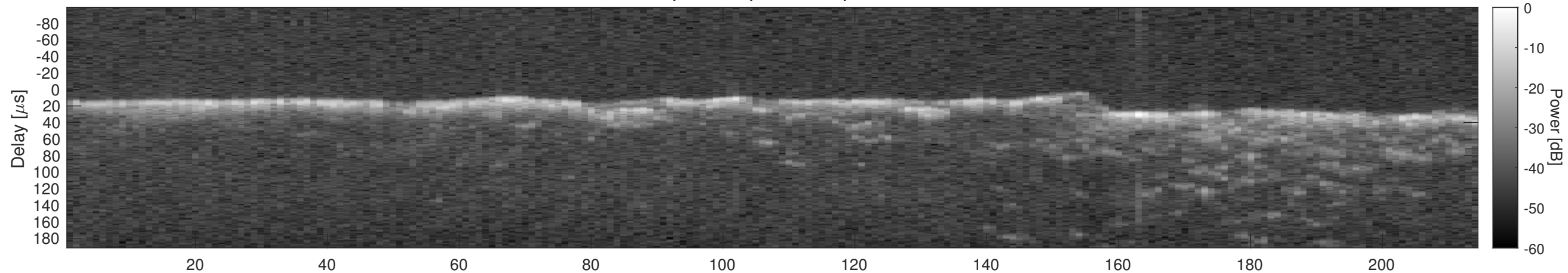
Orbit 8332, Window, Channel 2, Chapman
