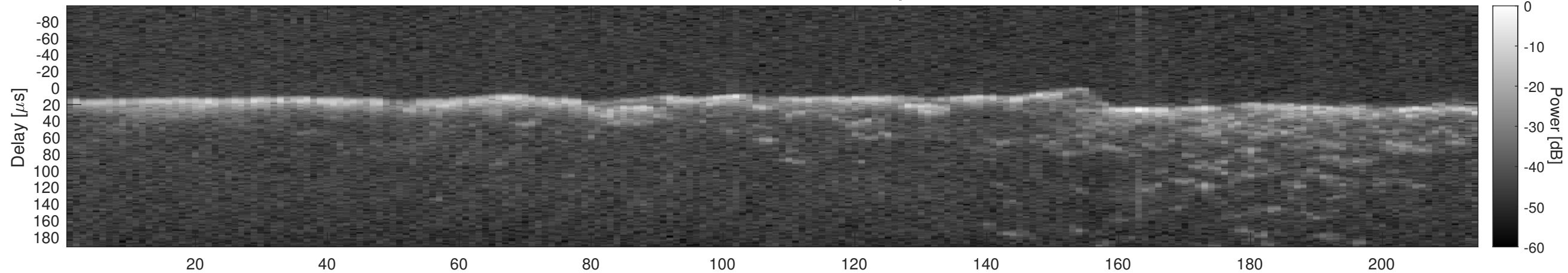
Orbit 8332, Window, Channel 2, Optimized
