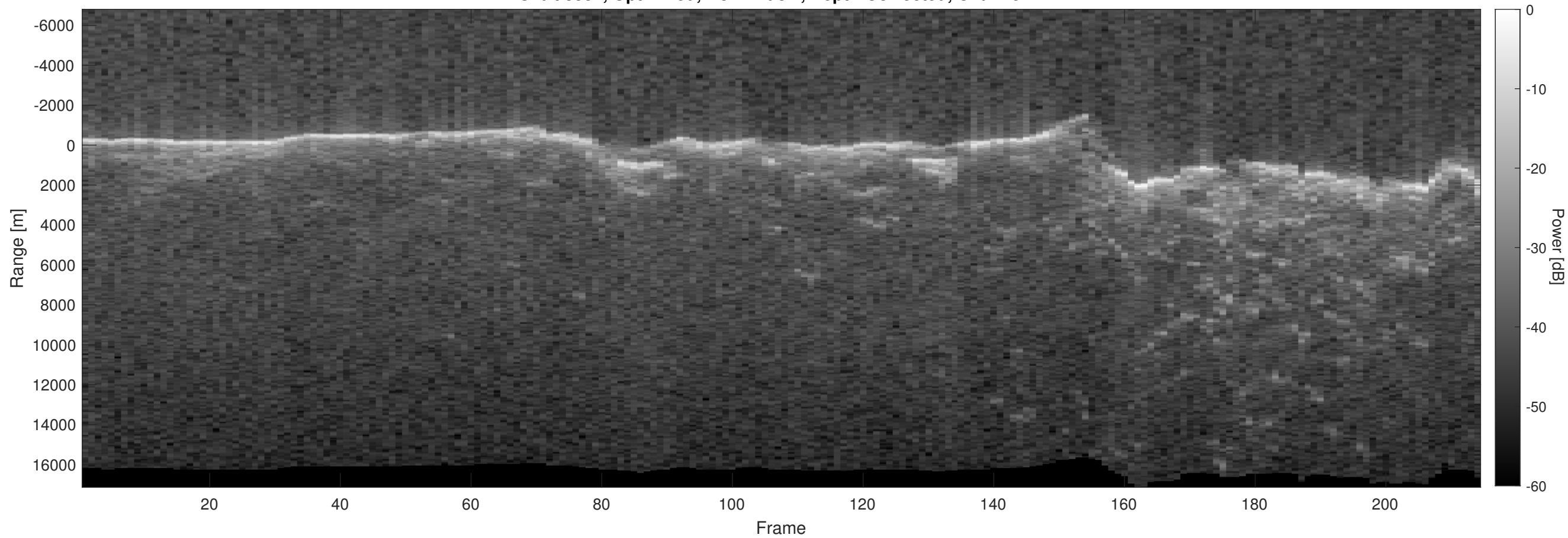
Orbit 8332, Optimized, No Window, Depth-Corrected, Channel 2
