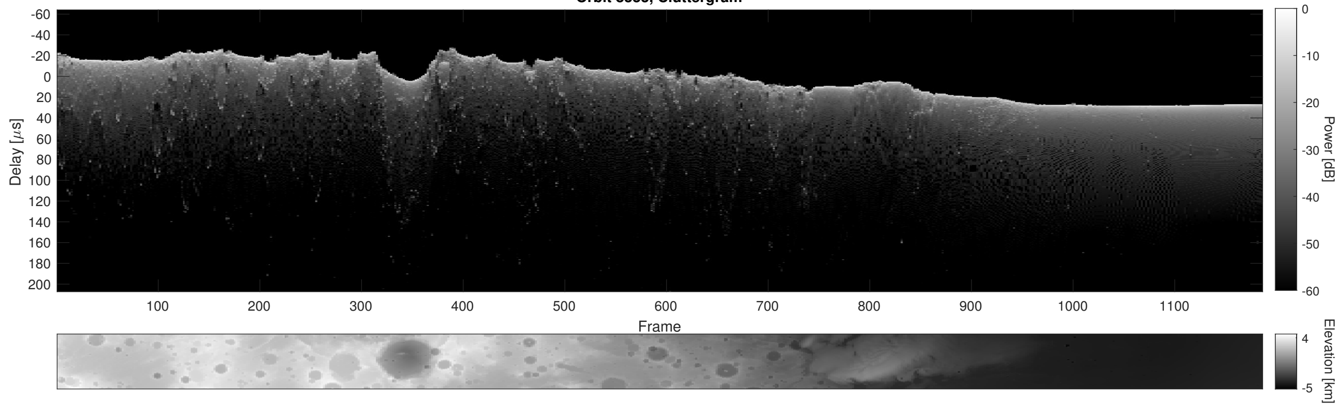
Orbit 8333, Cluttergram
