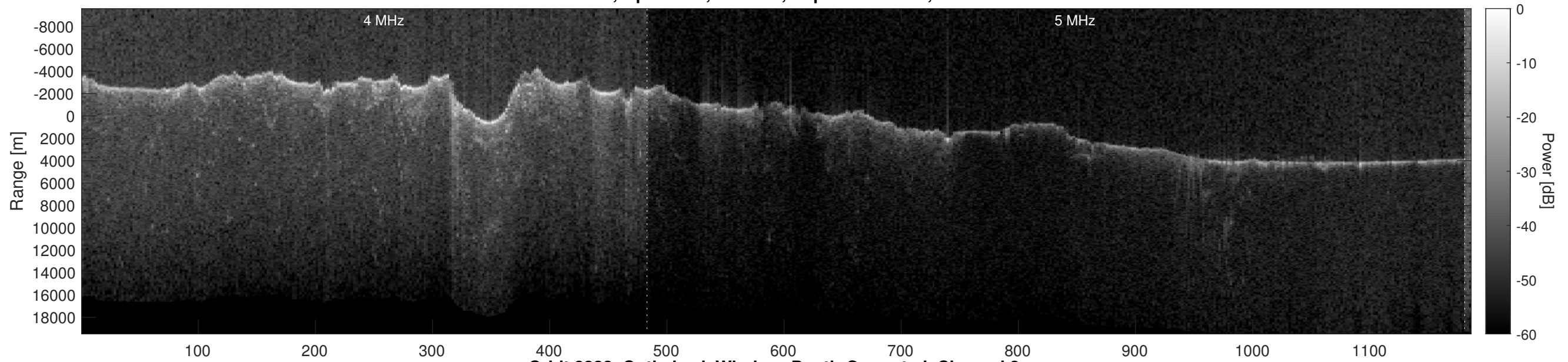
Orbit 8333, Optimized, Window, Depth-Corrected, Channel 2
