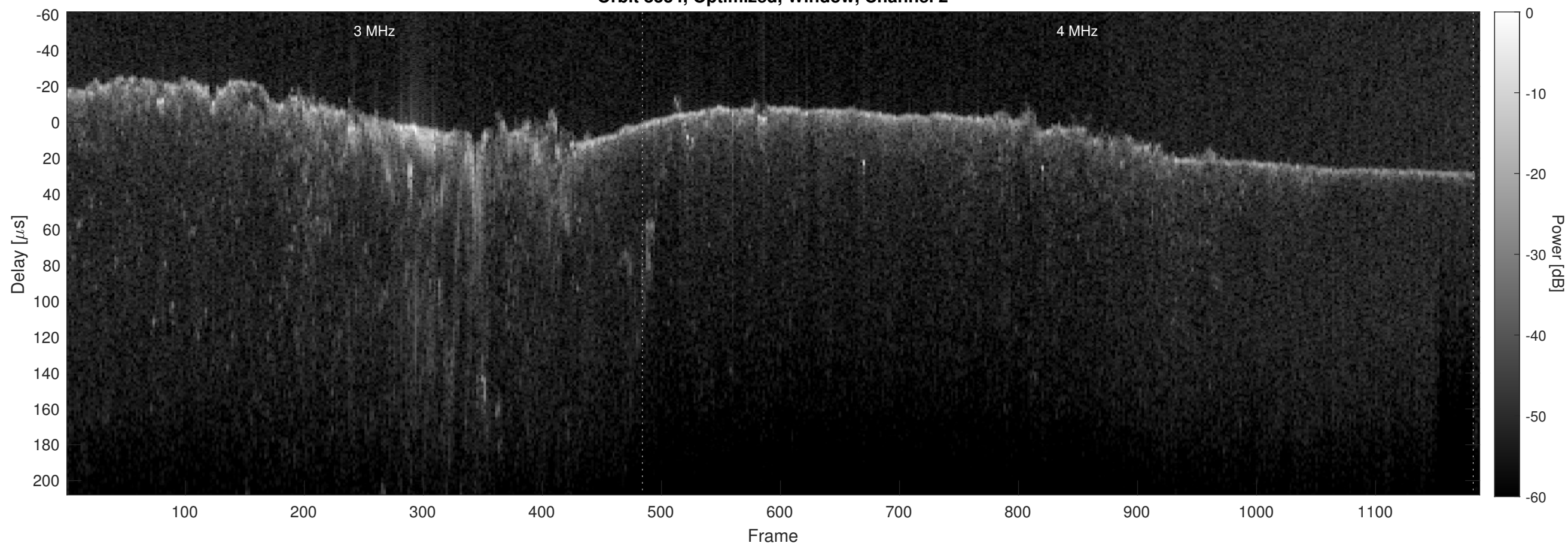
Orbit 8334, Optimized, Window, Channel 2
