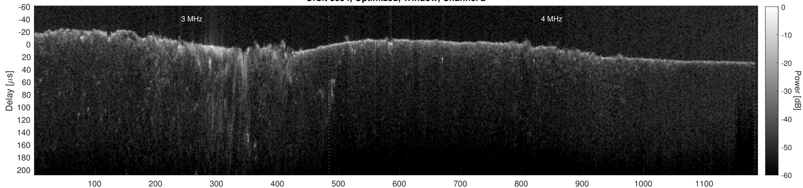
Orbit 8334, Cluttergram
