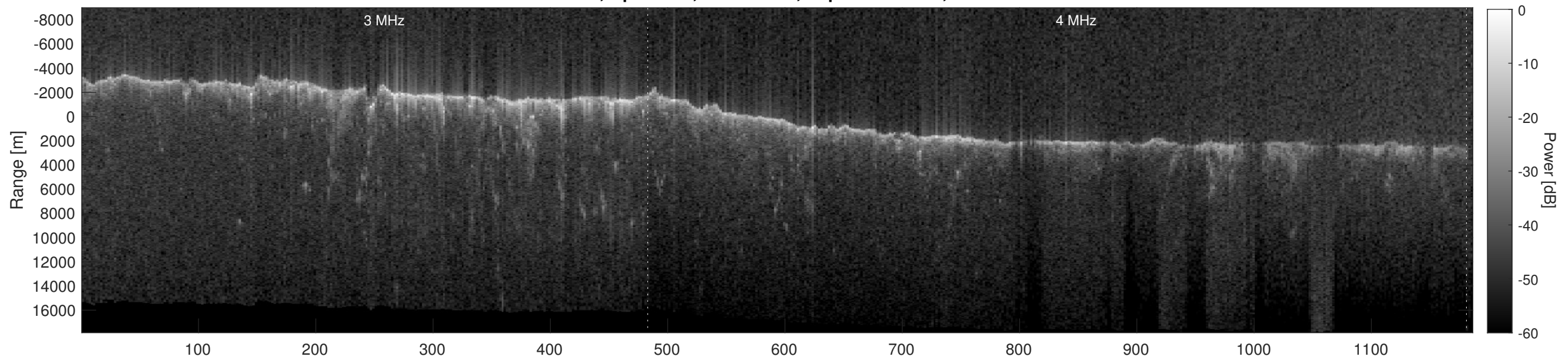
Orbit 8335, Depth-Corrected Cluttergram
