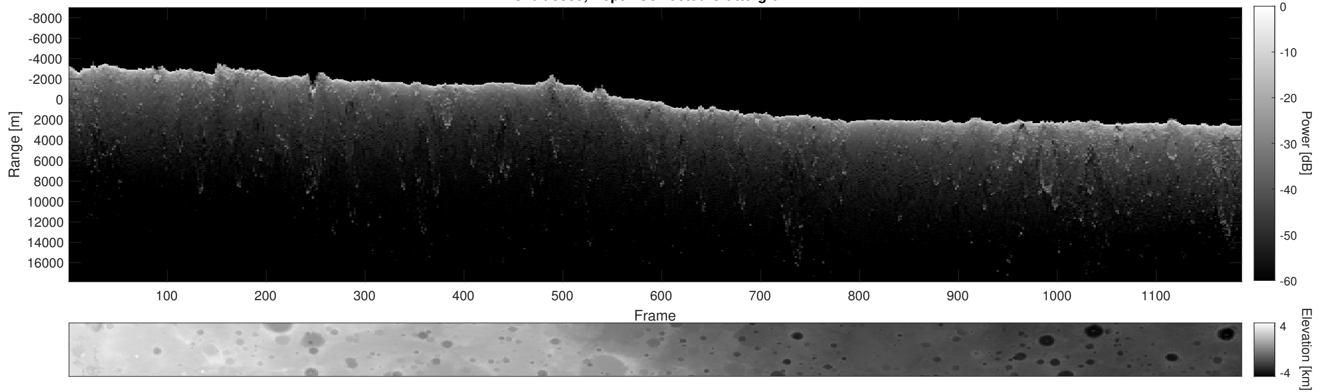
Orbit 8335, Depth-Corrected Cluttergram
