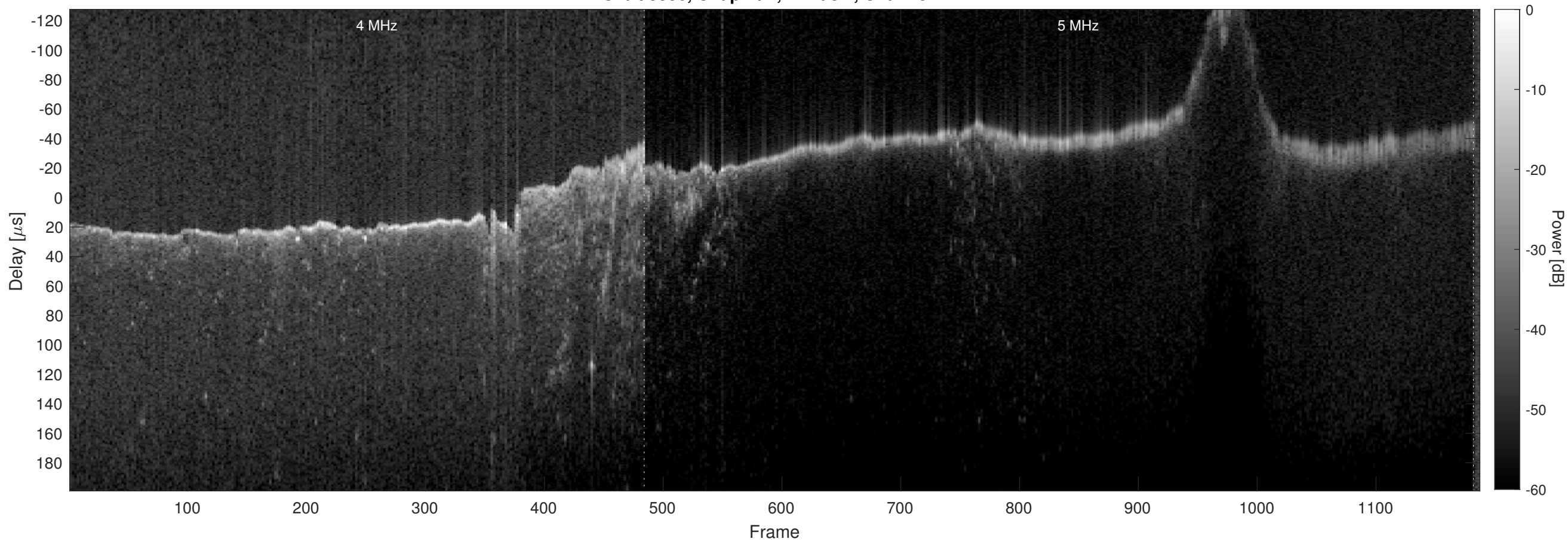
Orbit 8336, Chapman, Window, Channel 2
