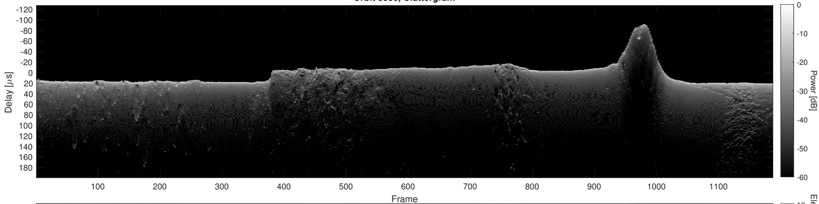
Orbit 8336, Cluttergram
