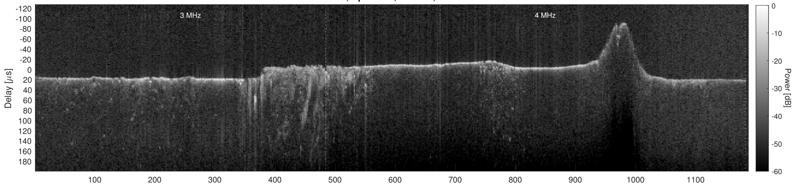
Orbit 8336, Cluttergram
