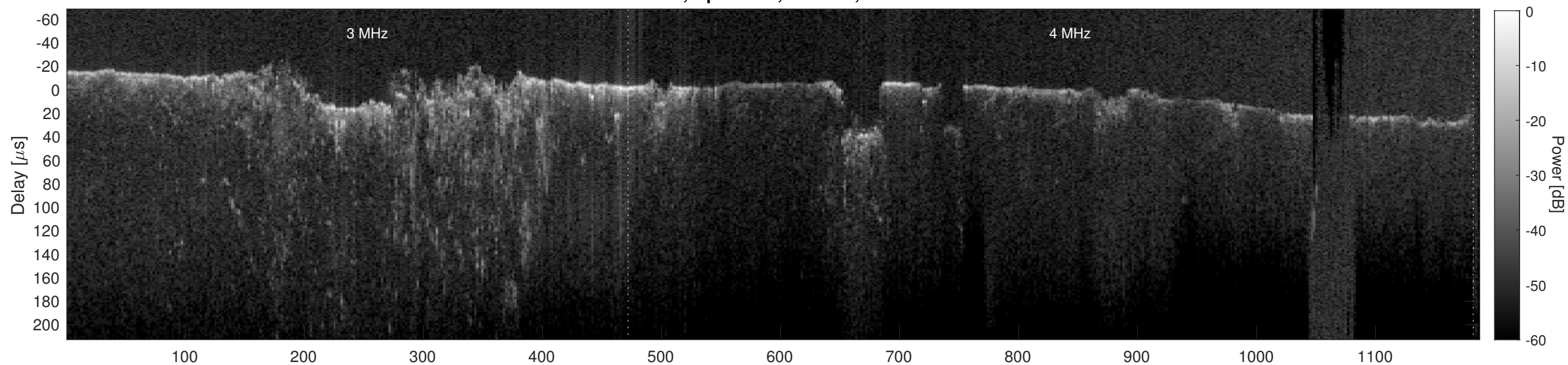
Orbit 8339, Cluttergram
