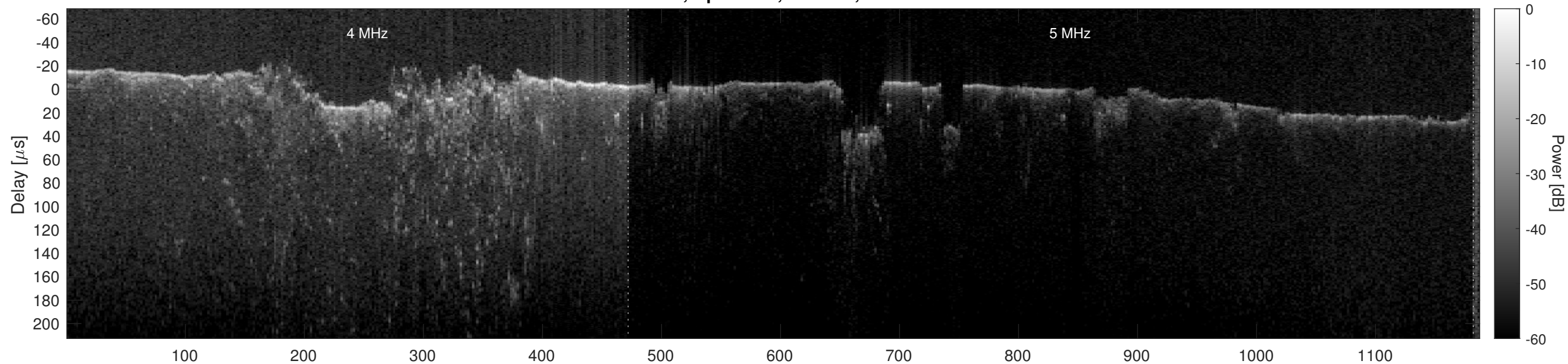
Orbit 8339, Optimized, Window, Channel 2
