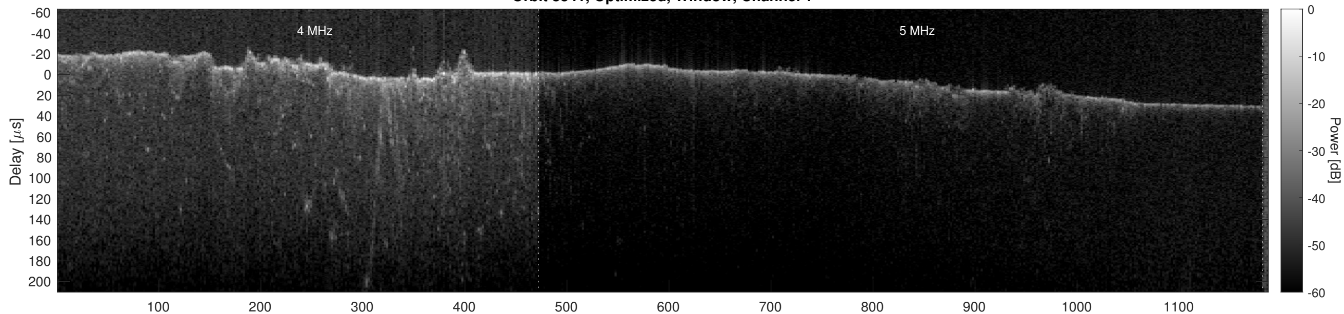
Orbit 8341, Optimized, Window, Channel 2
