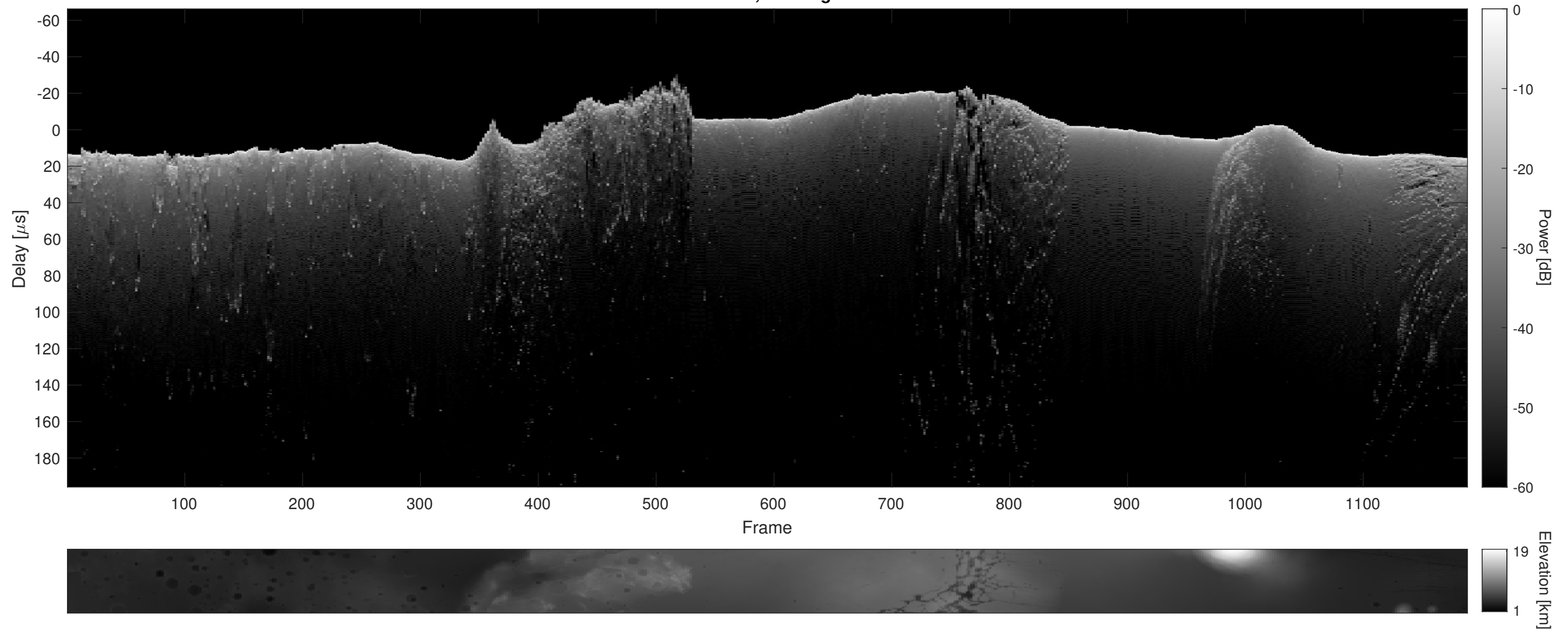
Orbit 8343, Cluttergram
