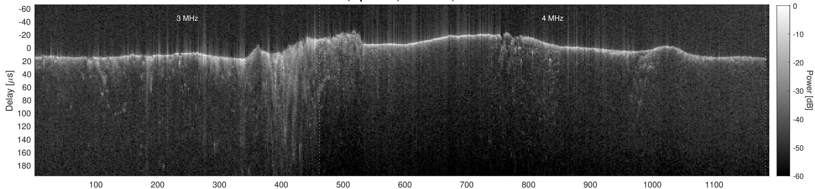
Orbit 8343, Cluttergram
