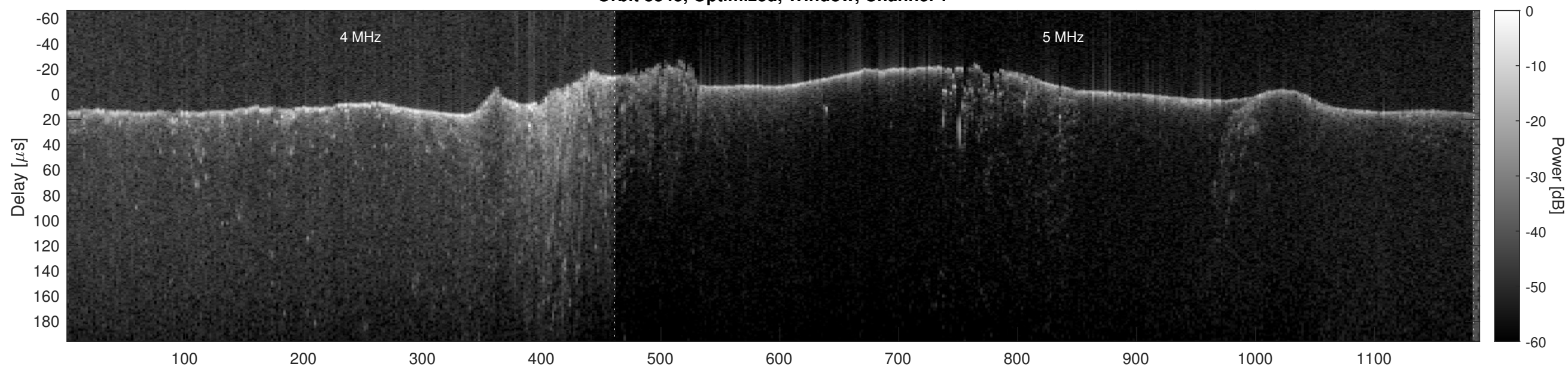
Orbit 8343, Optimized, Window, Channel 2
