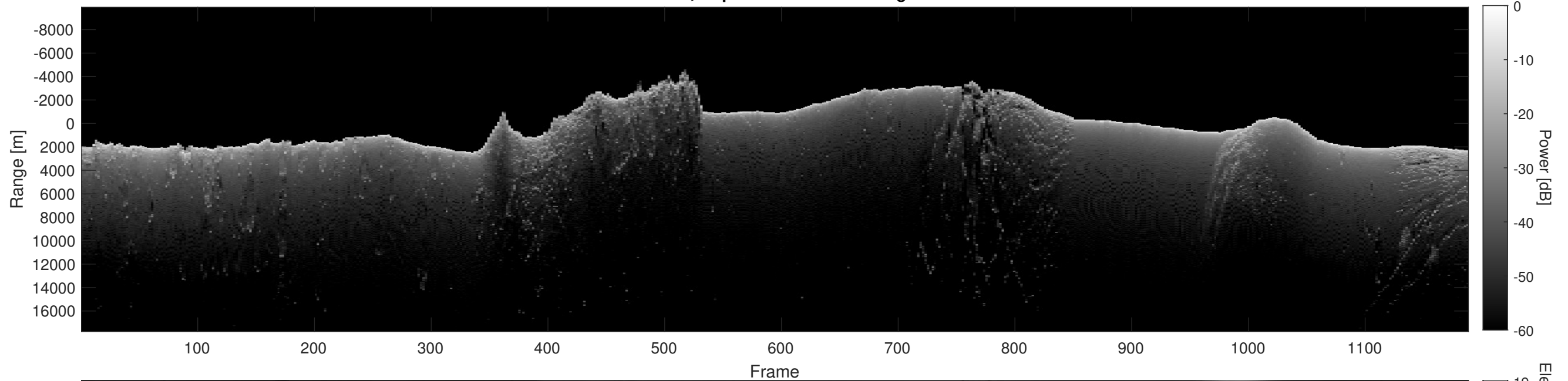
Orbit 8343, Depth-Corrected Cluttergram
