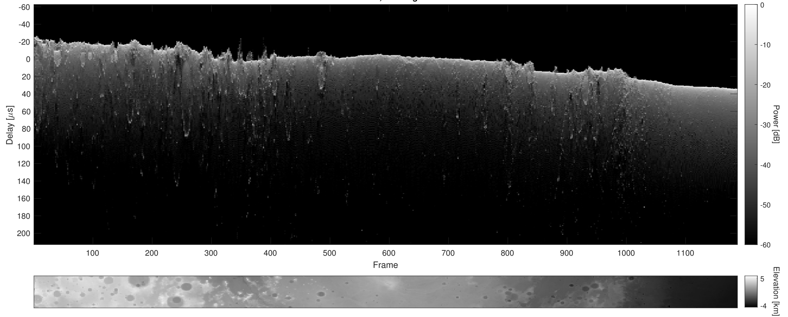
Orbit 8348, Cluttergram
