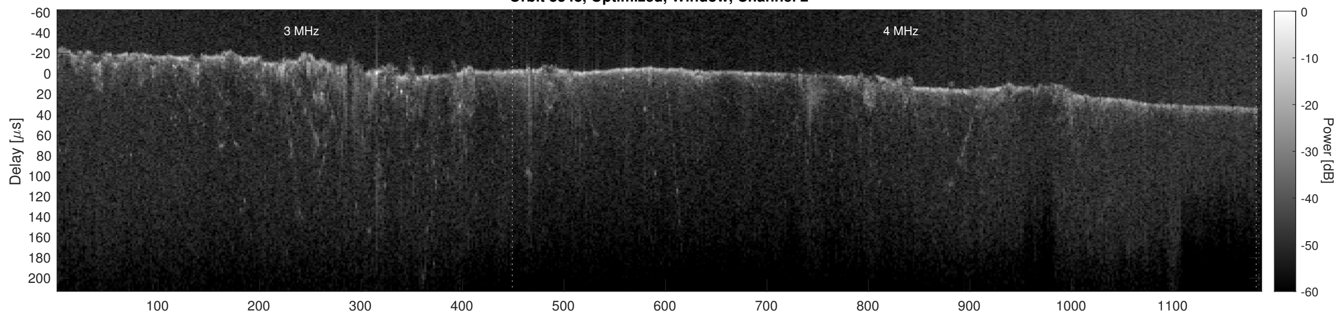
Orbit 8348, Cluttergram
