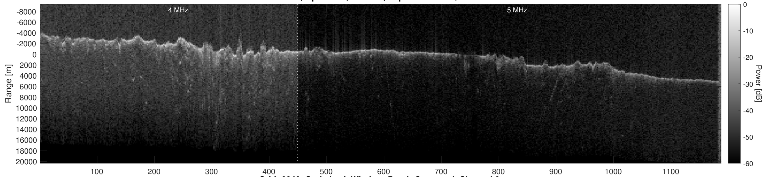
Orbit 8348, Optimized, Window, Depth-Corrected, Channel 2
