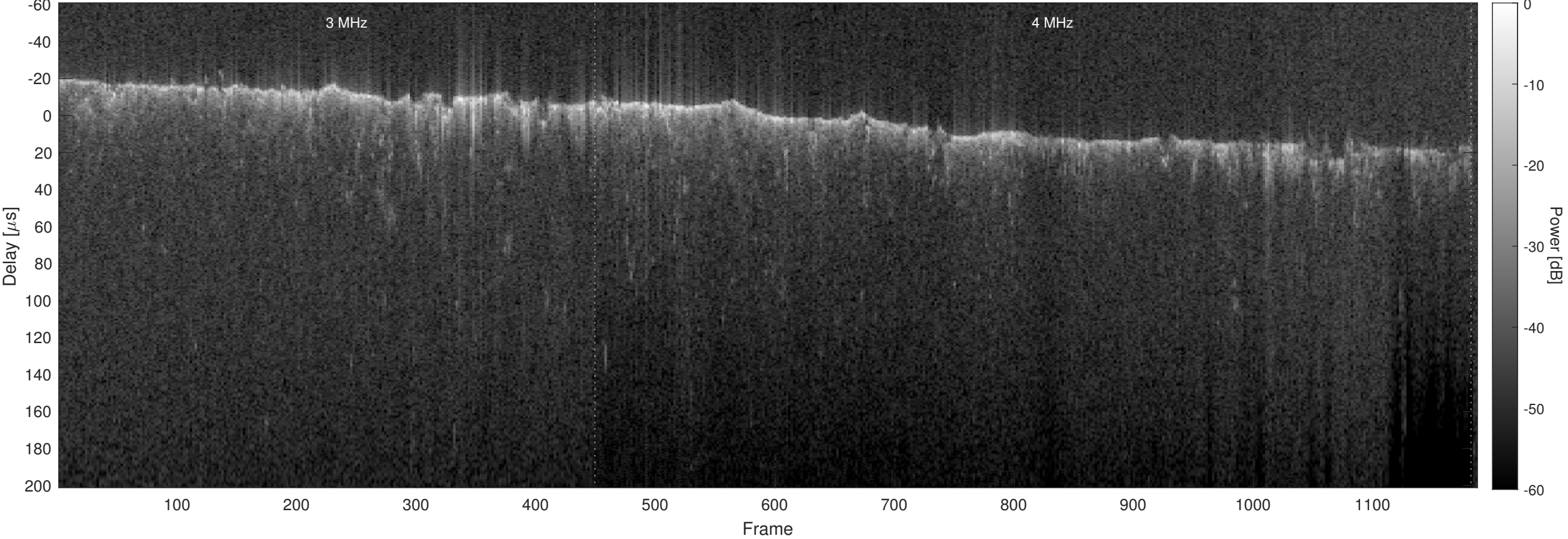
Orbit 8349, Optimized, No Window, Channel 2
