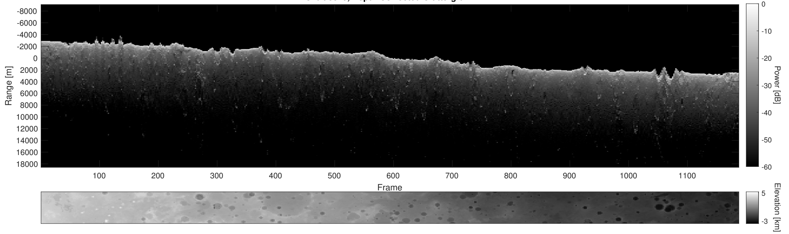
Orbit 8349, Depth-Corrected Cluttergram
