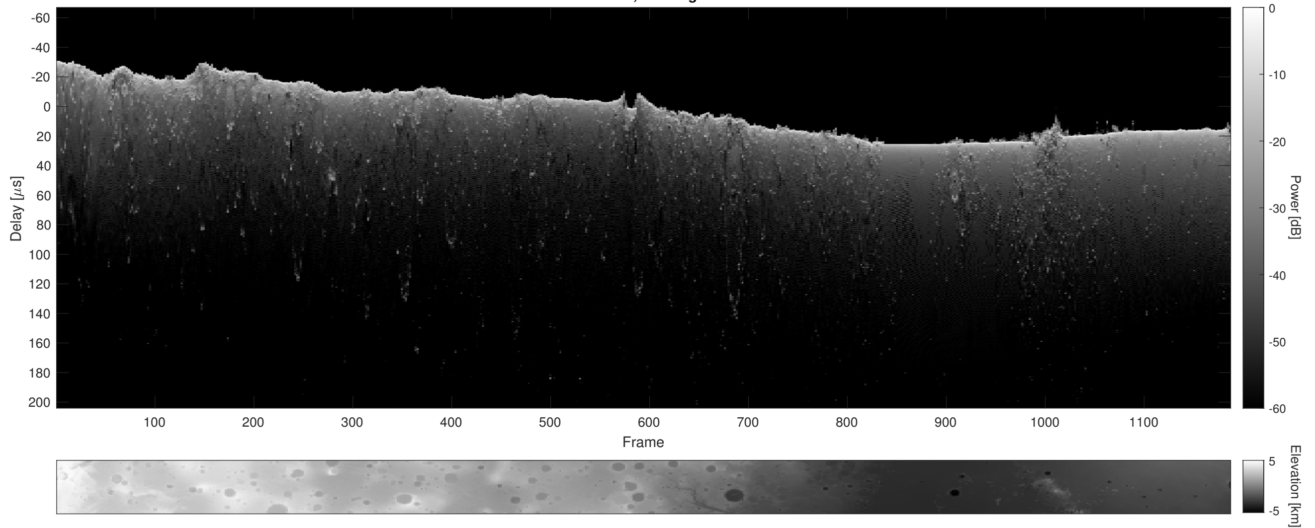
Orbit 8351, Cluttergram
