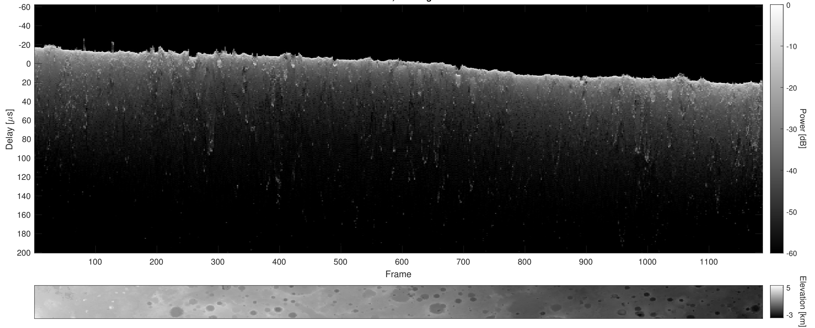
Orbit 8356, Cluttergram
