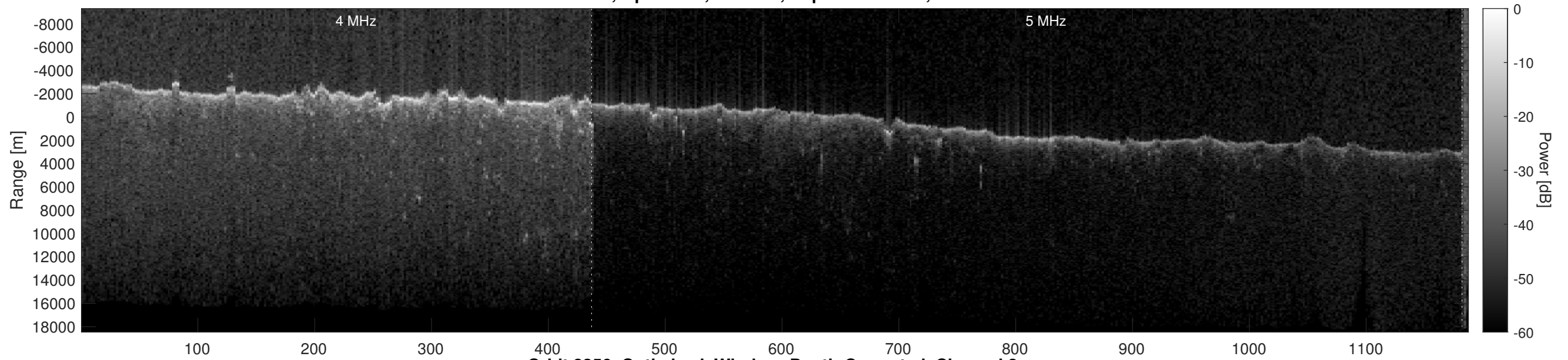
Orbit 8356, Optimized, Window, Depth-Corrected, Channel 2
