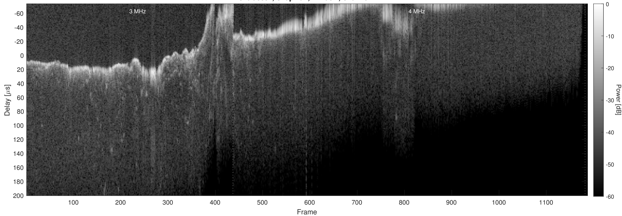
Orbit 8357, Chapman, Window, Channel 2
